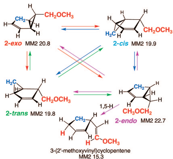
Figure 4. Thermal rearrangement of 6- exo -methoxymethylbicyclo[3.1.0]hex-2-ene ( 2- exo ) to the other three products of the system, and the ultimate product, 3-(2'-methoxyvinyl)cyclopentene, are shown. Included are calculated steric energies in kcal mol -1 .
