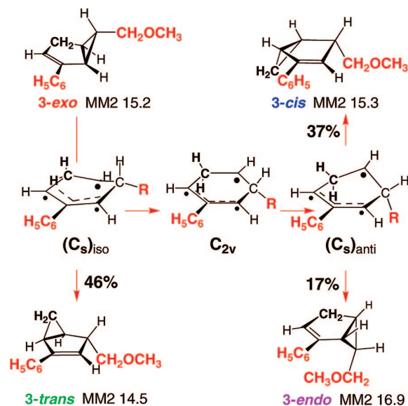
Figure 5. Thermal rearrangements of 2-phenyl-6- exo -methoxymethylbicyclo[3.1.0]hex-2-ene ( 3- exo ) to 3- trans , 3- cis , and 3- endo at 216.5 °C are shown. Included are MM2 steric energies in kcal mol -1 .
